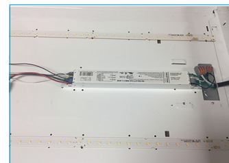
S44: Driver & 12VDC Output
