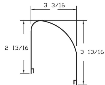
DIFFUSER
