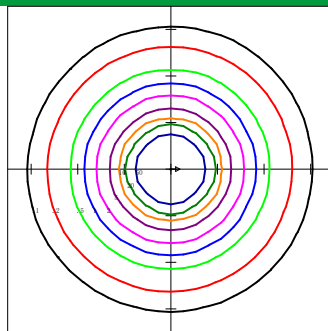
HBUF-200W-40-G4-B FIXED
