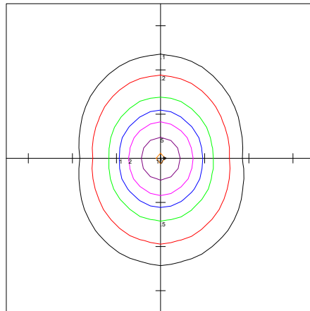
LNS-4FT-25-T1-F @10FT Set At 30W,5000K Distribution@10FT
