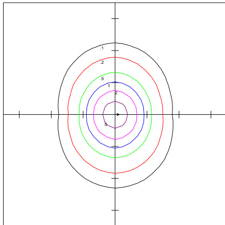
LNS-4FT-25-T1-F @10FT Set At 25W,5000K Distribution@10FT
