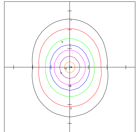
LNS-4FT-25-T1-F @10FT Set At 40W,5000K Distribution@10FT
