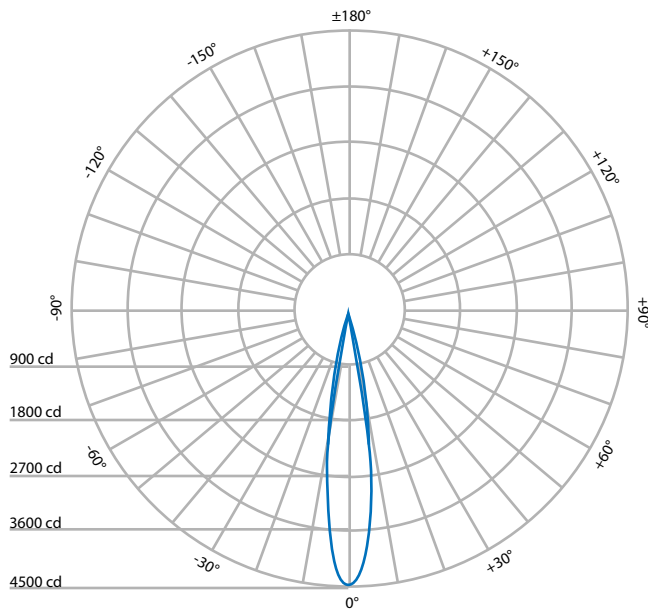
Polar Distribution Chart (units in Candela - cd)
