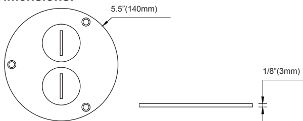
Cover Plate
