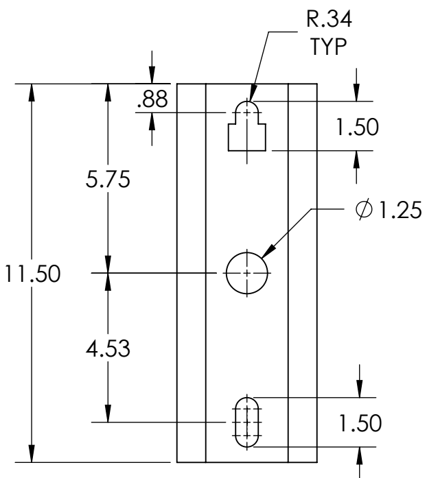
MOUNTING PLATE (EPB-MP)
