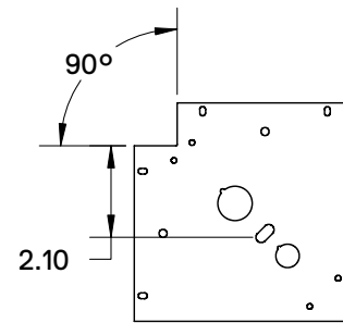
90° Bracket
