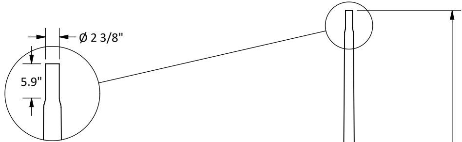
Standard Pole Top with 2 3/8" Tenon
