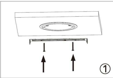
Fixing bracket on terminal box;
