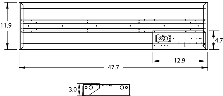
1x4 Dimensions
