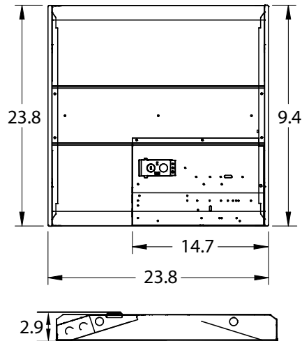
2x2 Dimensions
