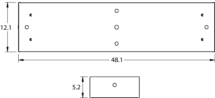
1x4 Surface Mount Dimensions
