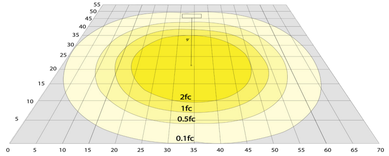
Area 55'x 70' Mounting Height: 9'
