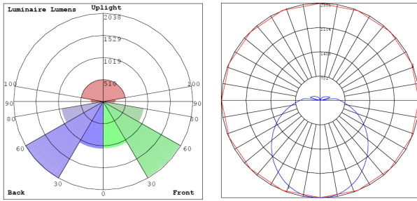
BUG Rating: B3-U4-G3
