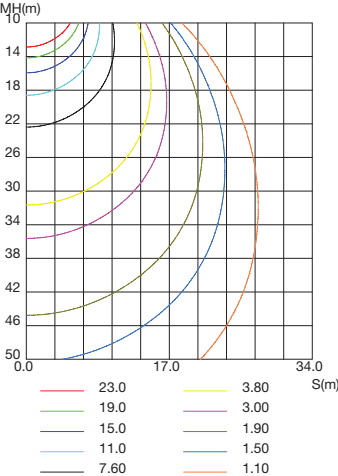
C0 PLANE ISOLUX DIAGRAM (UNIT:lx)
